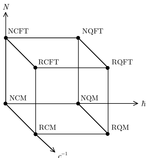
Figure 2. Relations between theories in the absence of gravity.
